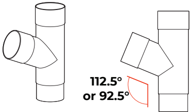
112.5° branch shown
