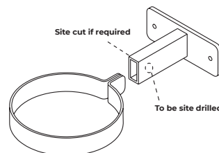
Tee bracket
