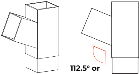
112.5° branch shown
