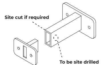
Tee Bracket
