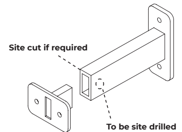
Mullion Bracket
