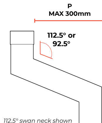
112.5° swan neck shown
