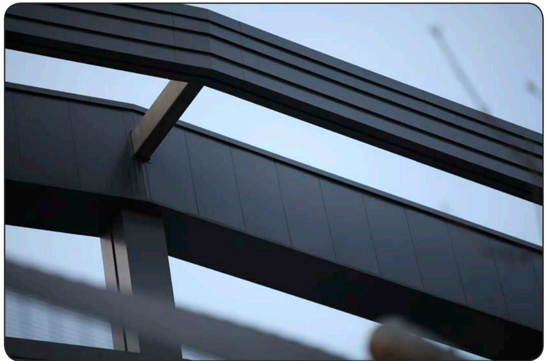
Combination of Vertical Arrowhead Boards, Fascia Panels, Soffit Planks and Copings to Clad The Flying Beams. Column Casings too.
