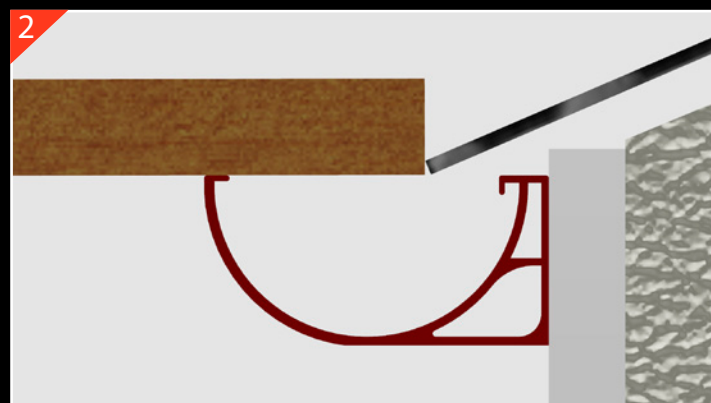
Alternatively use a spirit level against the lowest point of the roof tile to determine the position of the fascia bracket . *
