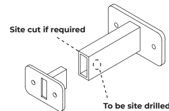
Tee Bracket
