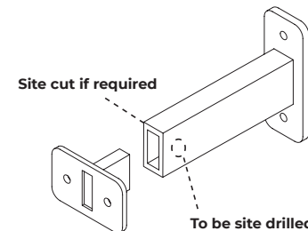
Mullion Bracket
