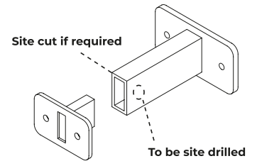
Tee Bracket
